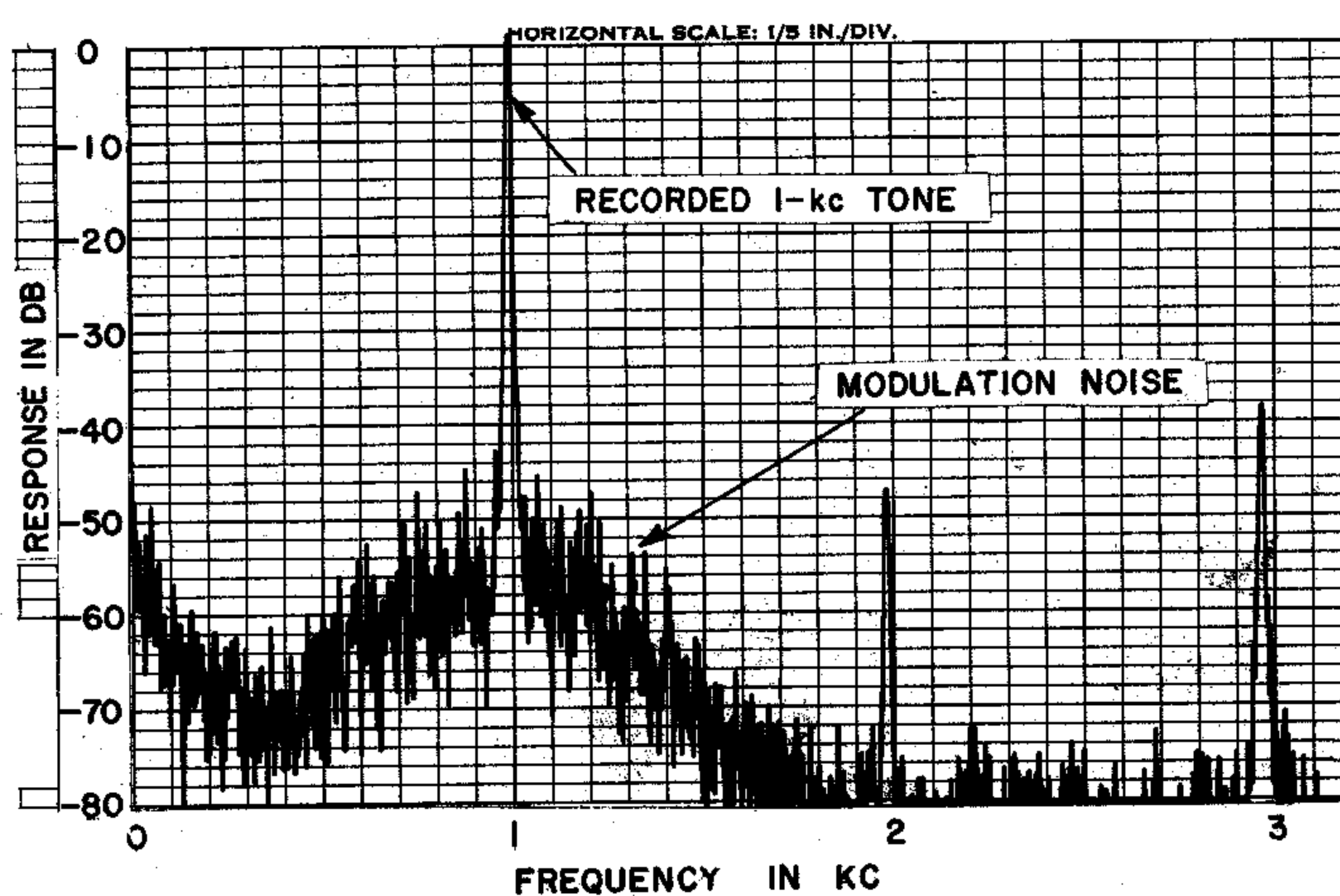
Figure 3-2. Charts of modulation noise on a 1-kc tone for two different types of magnetic tape. Note that one is about 10 db better than the other. Such measurements can be made easily with the recording analyzer, due to its 80-db dynamic range. For these records, chart speed was 2.5 inches per minute; writing speed, 10 inches per second; bandwidth, 10 cps.
