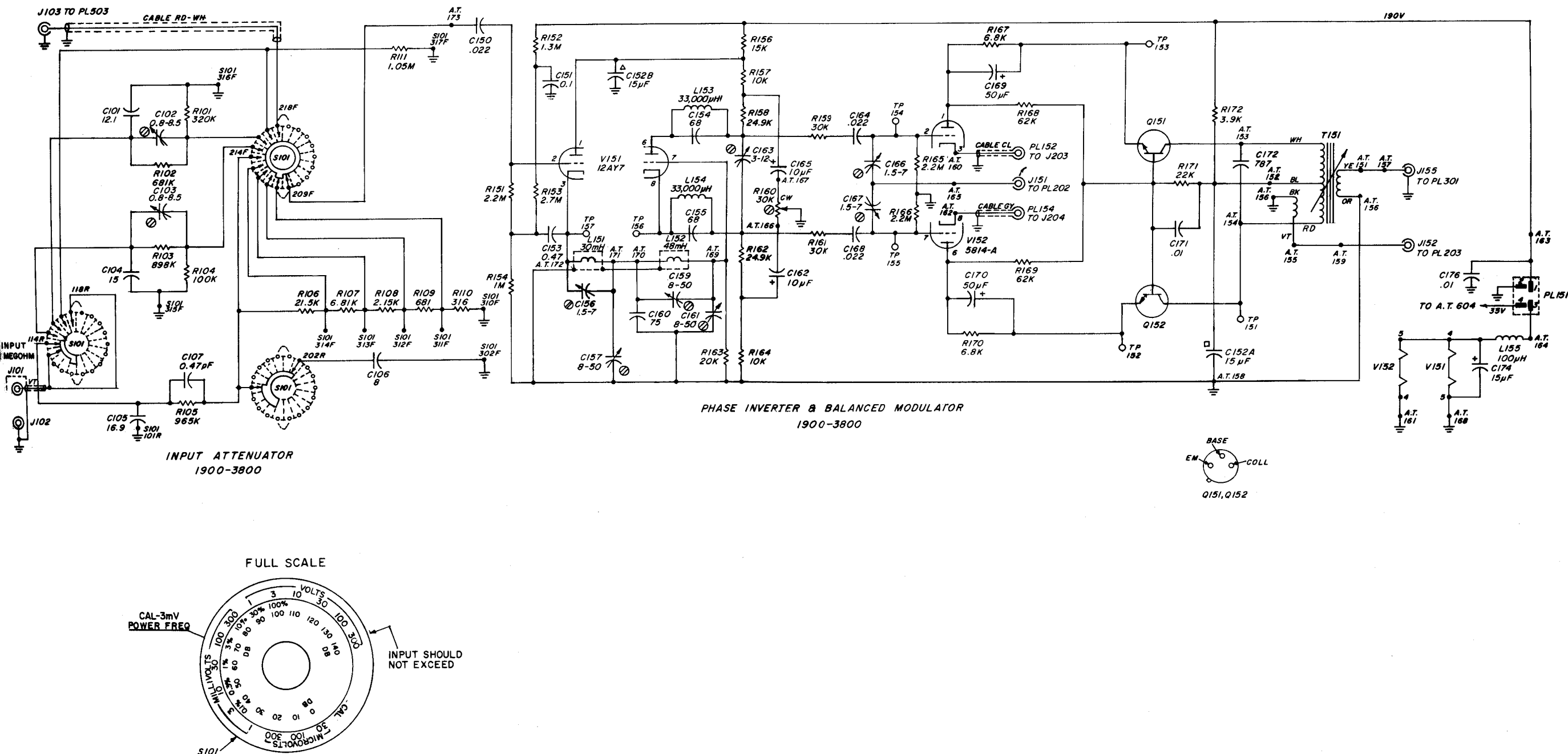
Figure 6-24. Schematic diagram for the input-section circuits.
