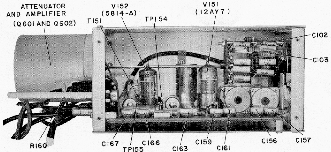
Figure 6-22. Input section.
