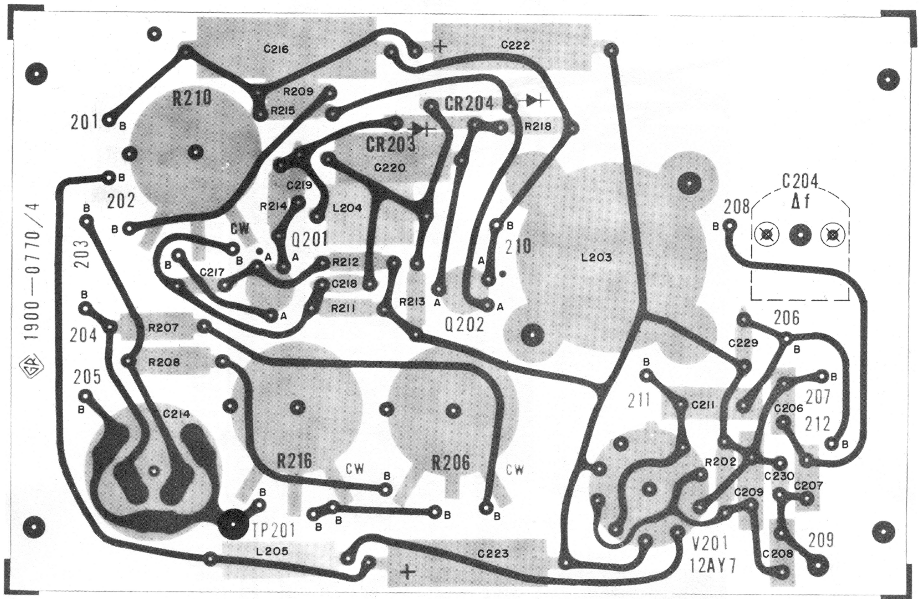
Figure 6-10. Etched-board layout for the variable oscillator.
