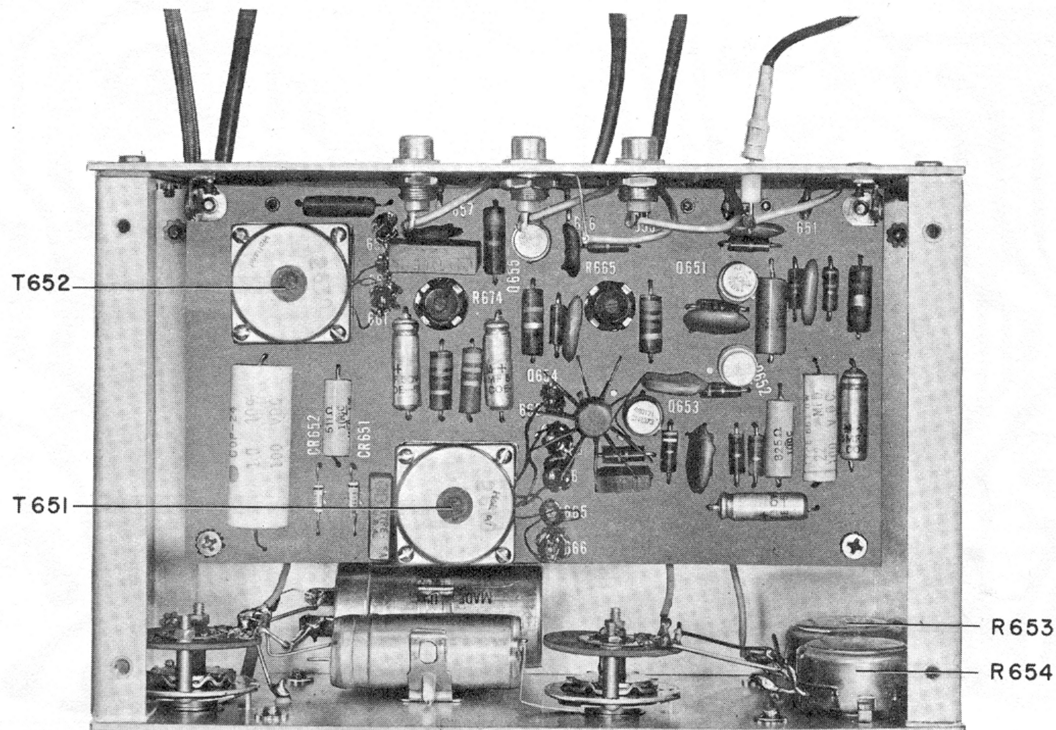
Figure 6-14. Output amplifier.
