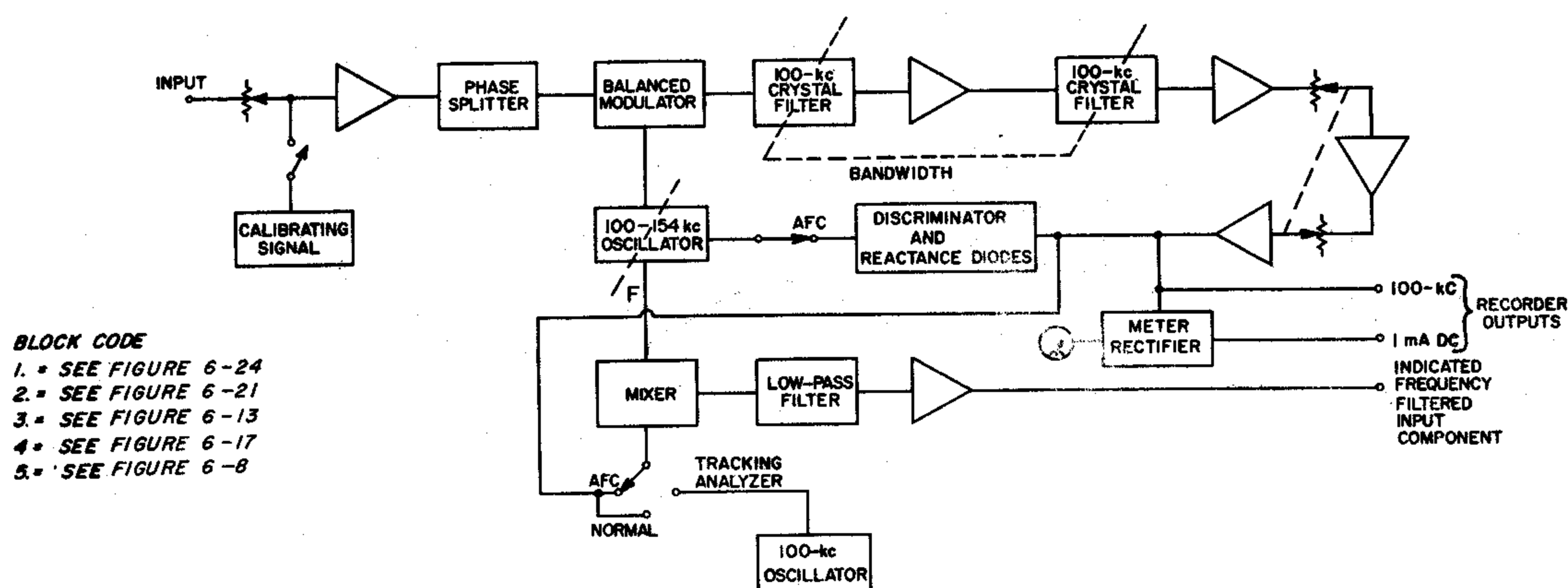
Figure 1-2. Block diagram of the analyzer.
