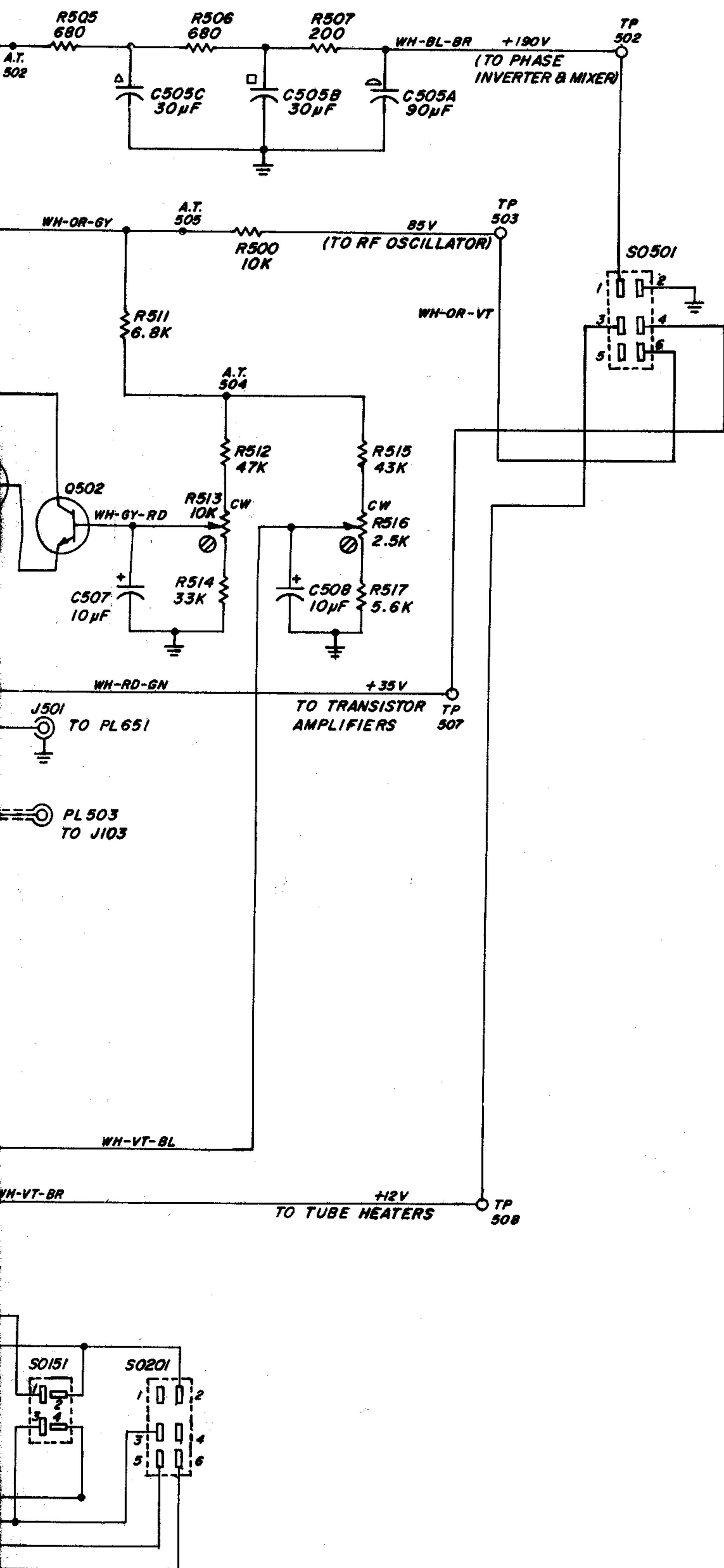
Figure 6-8. Schematic diagram of the power-supply circuits.
