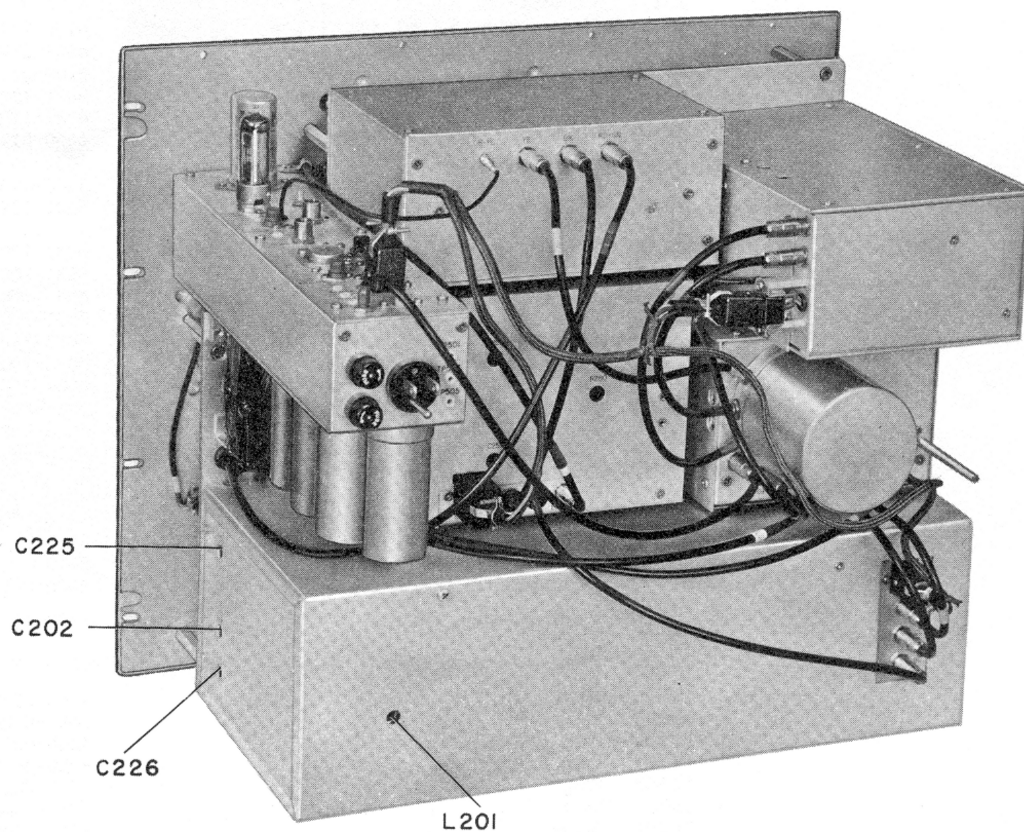
Figure 6-6. Interior view of the analyzer showing adjustments for the variable oscillator.
