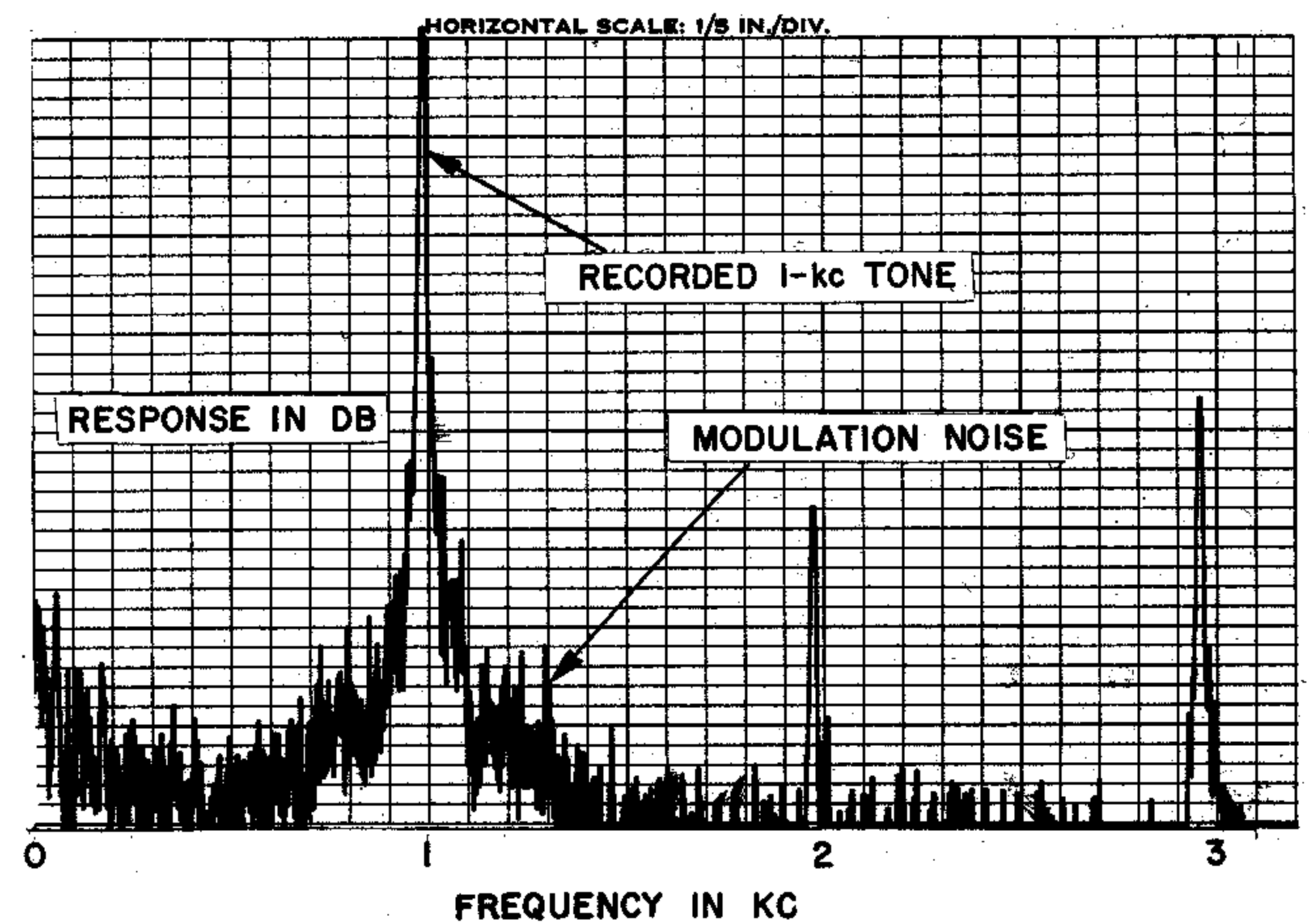
Figure 3-2. Charts of modulation noise on a 1-kc tone for two different types of magnetic tape. Note that one is about 10 db better than the other. Such measurements can be made easily with the recording analyzer, due to its 80-db dynamic range. For these records, chart speed was 2.5 inches per minute; writing speed, 10 inches per second; bandwidth, 10 cps.
