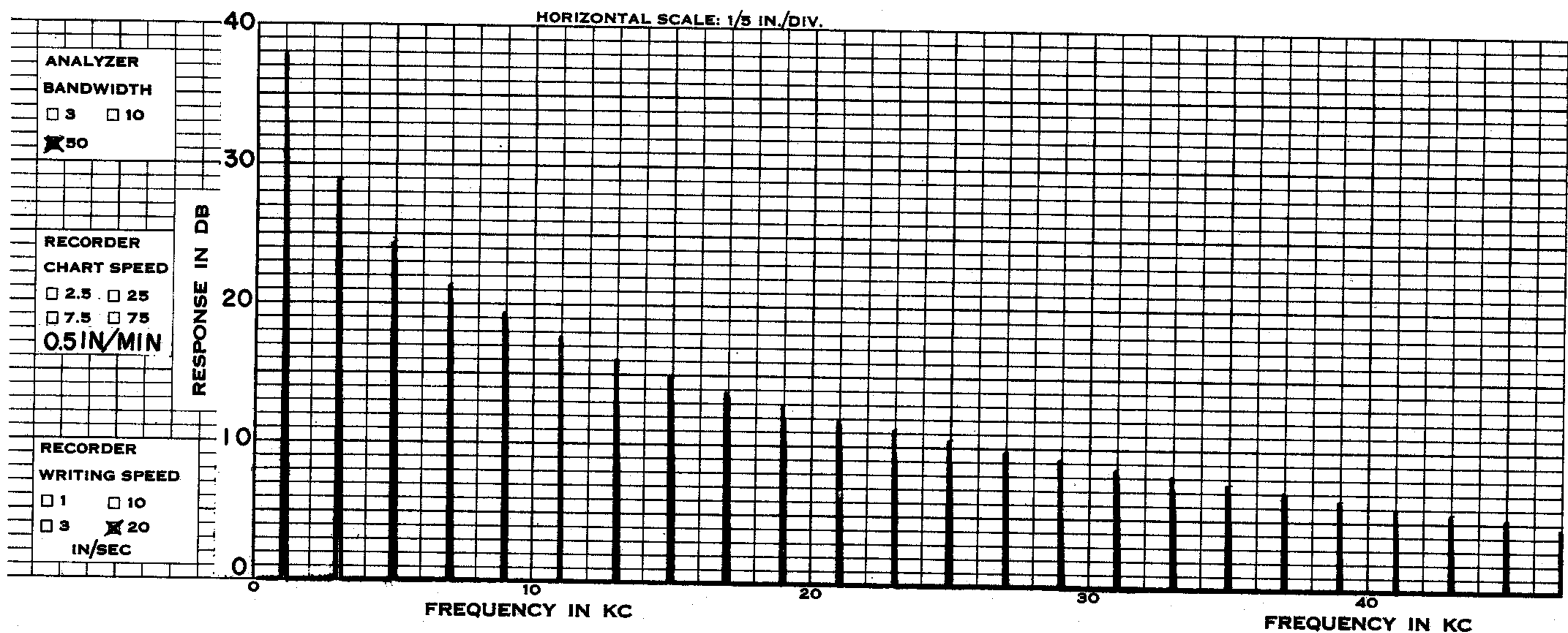
Figure 5-1. The harmonic components of a 1-kc square wave. The absence of even harmonics shows that the wave is symmetrical.
